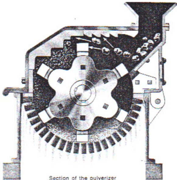
Section of the pulverizer
